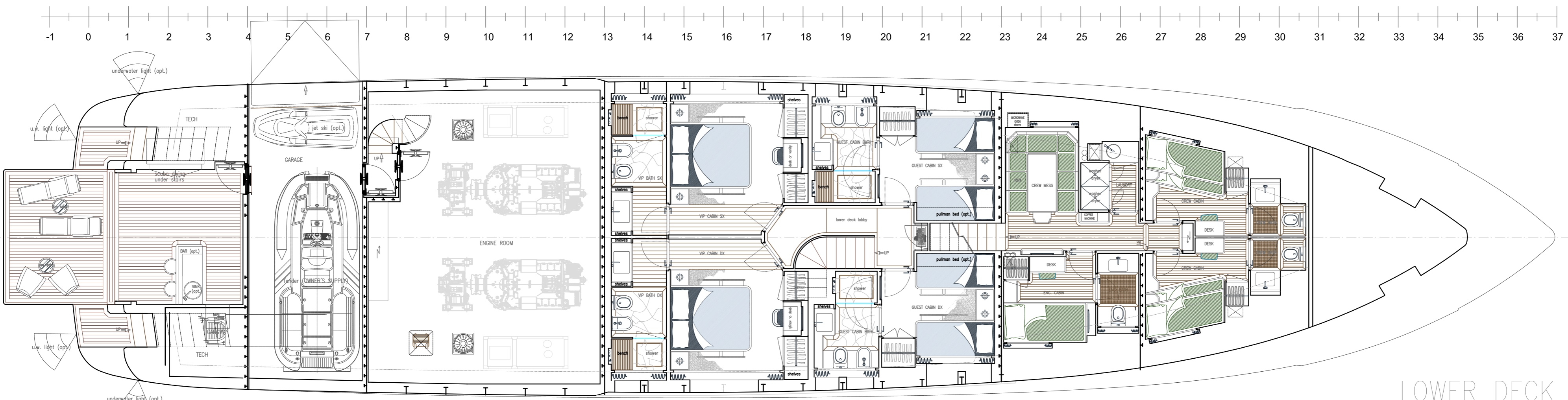
MAIN DECK
