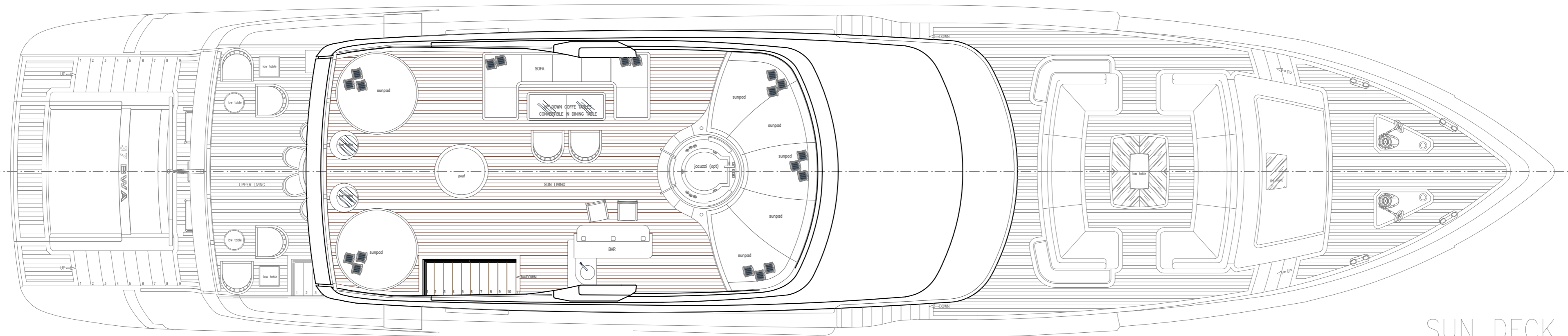
SUN DECK
