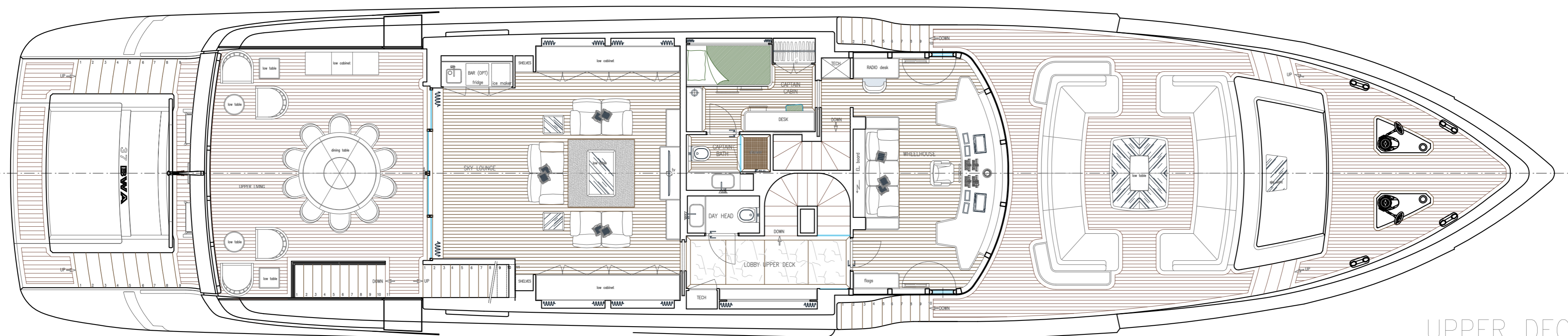
UPPER DECK
