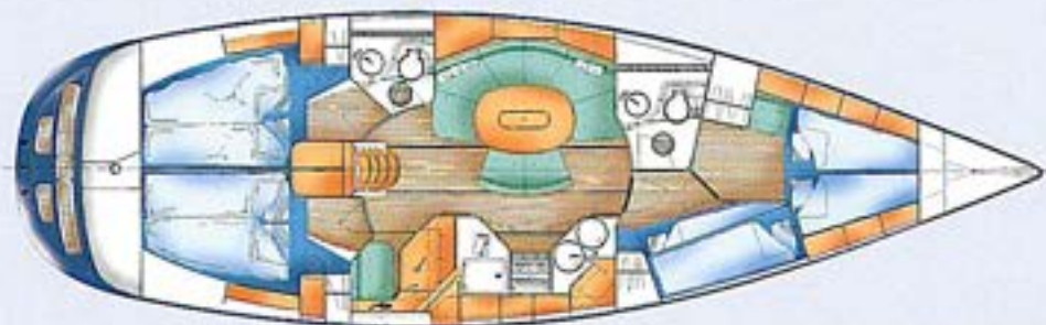
4 CABIN ACCOMMODATION
