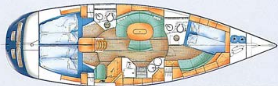
3 CABIN ACCOMMODATION
