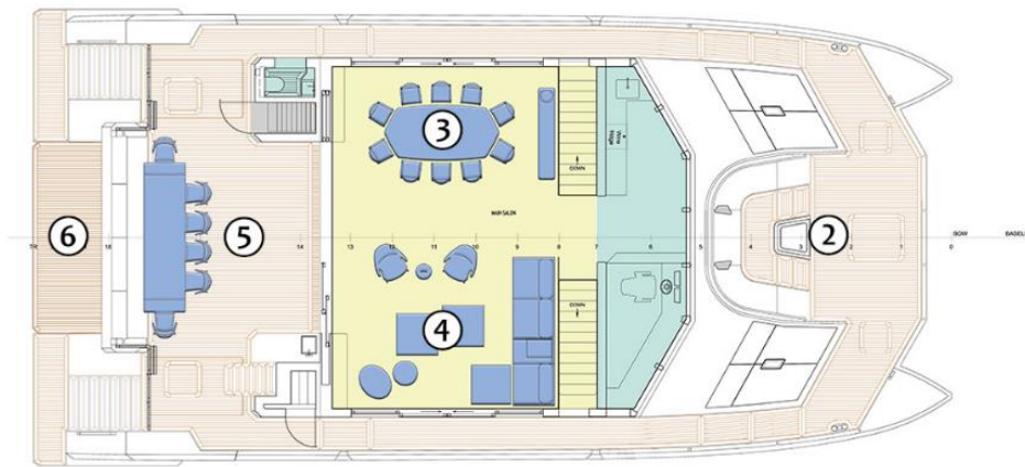
MAIN DECK
