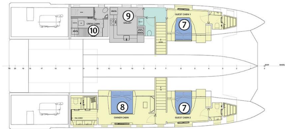
LOWER DECK
