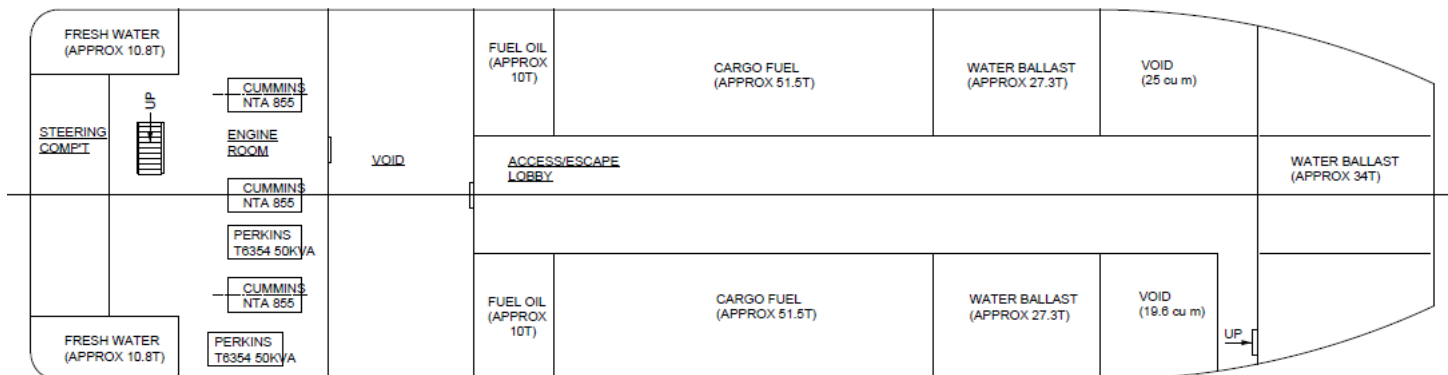
UNDER DECK PLAN
