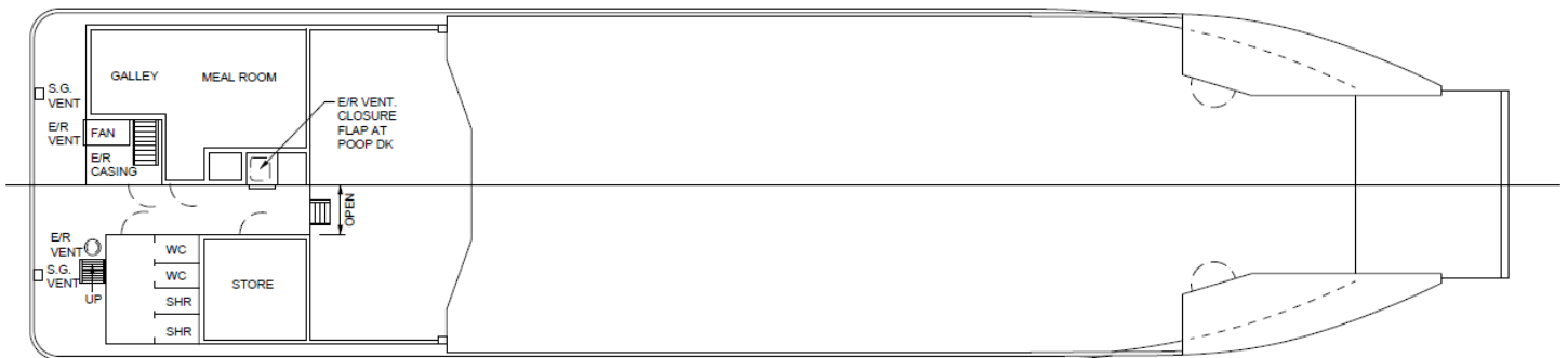
WEATHER DECK PLAN
