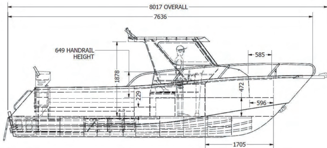
PROFILE SCALE 1:35
